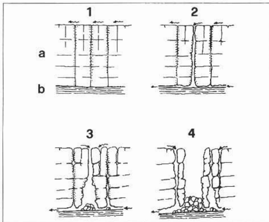
Fig. 6 - Evolution of a sima: a) coarse arenite; b) medium-fine arenite. See the text for explanations.
