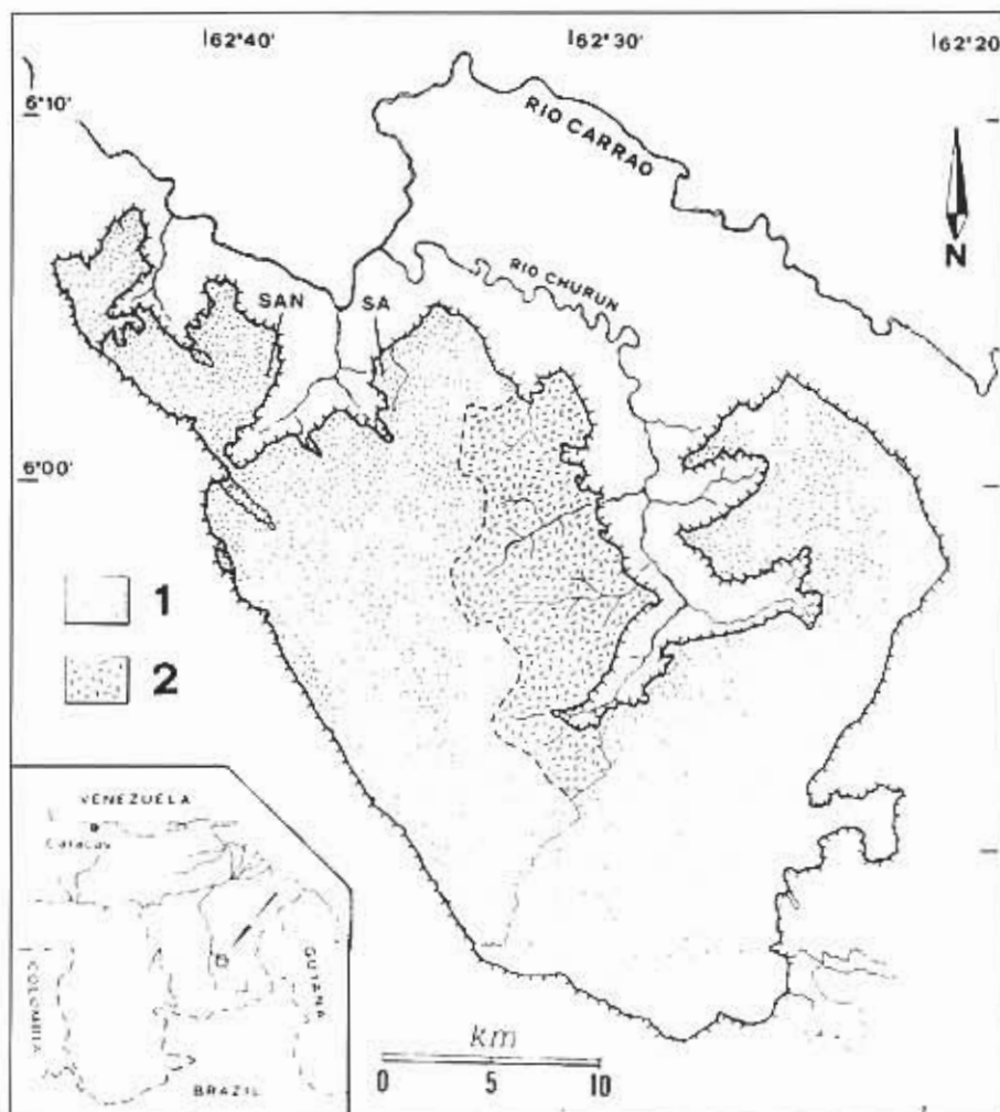
Fig. 1 - Location map of the Auyàn-tepui and the investigated areas: SAN = Sima Auyàn-tepui Noroeste, SA = Sima Aonda. 1) Siliceous arenites (Mataui Formation), 2) Approximative outcropping of diabase.
